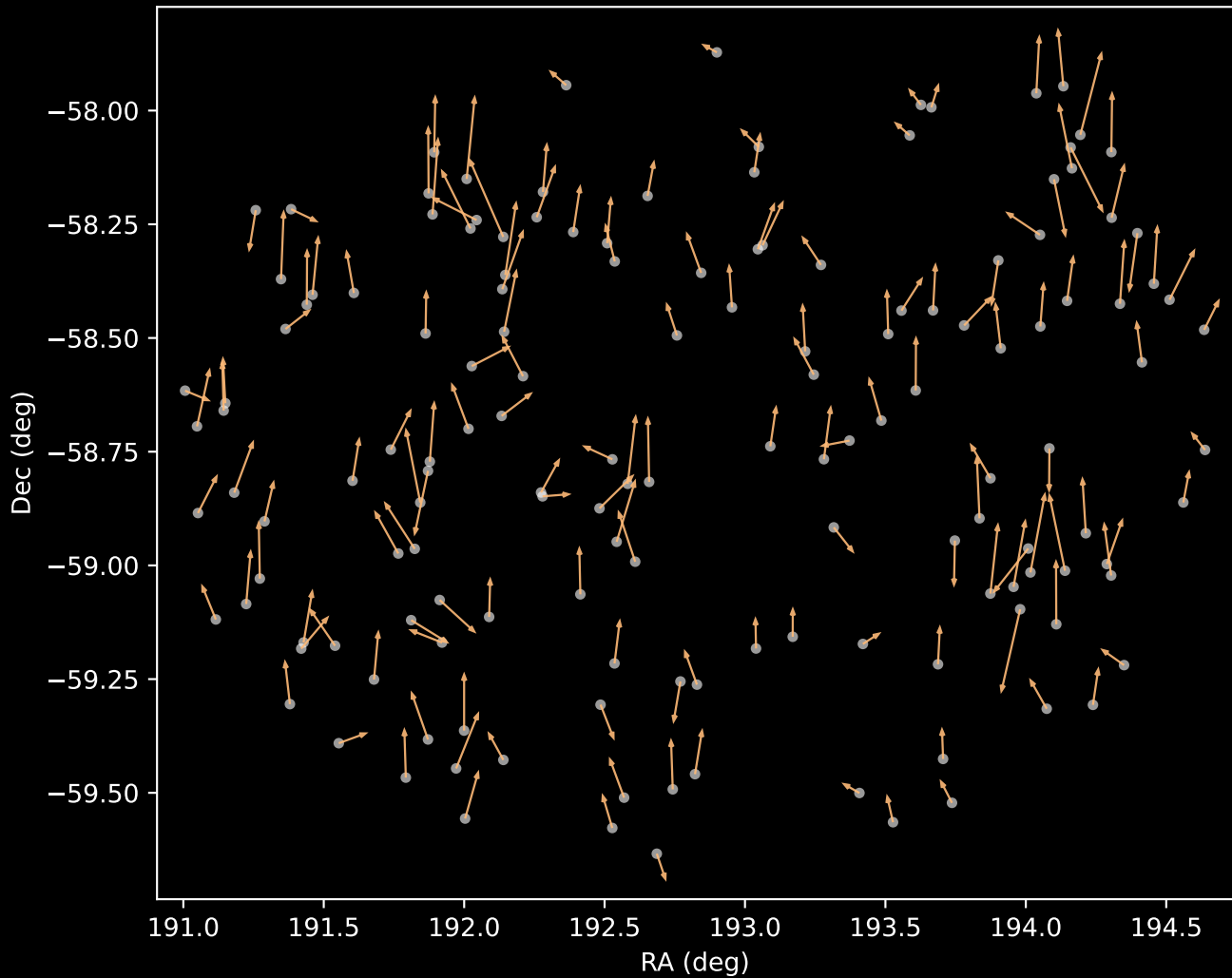
GALAH DR4 Cluster 3 Proper Motion Vectors (n=150)
