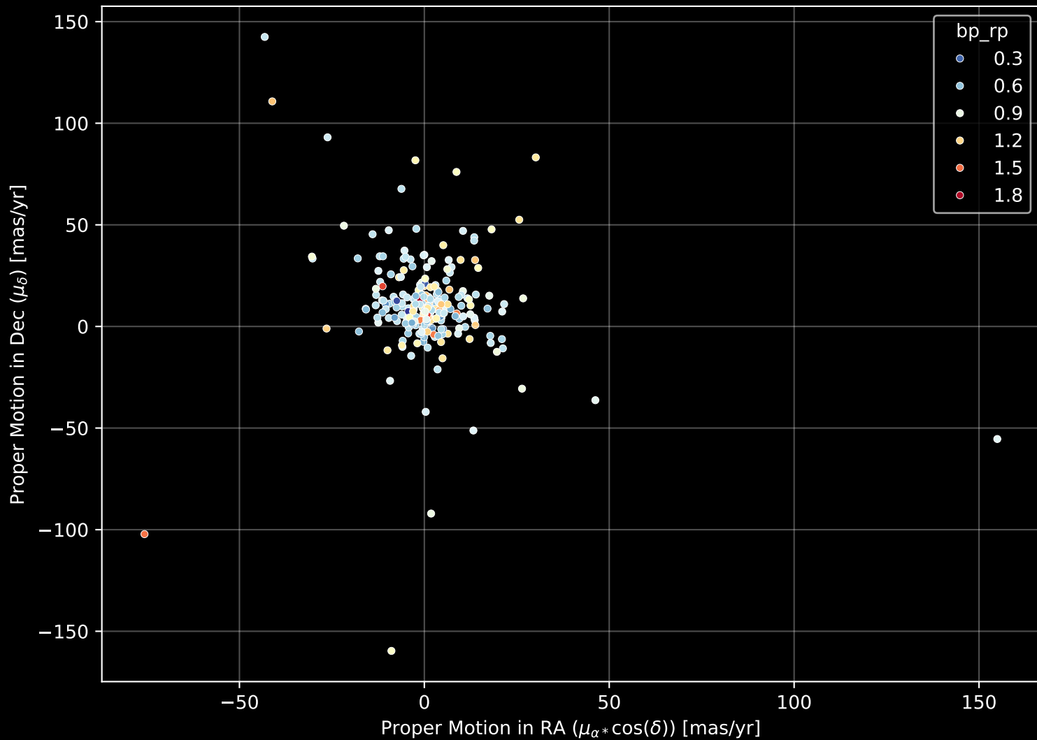
GALAH DR4 Field: [7161] Proper Motion Diagram (n= 241)
