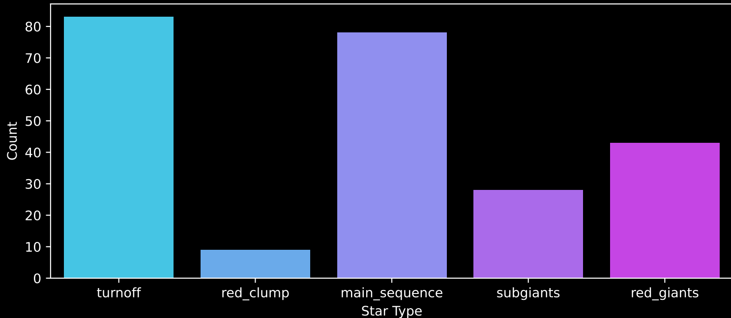
GALAH DR4 Field: [7161] Count plot of Star Type
