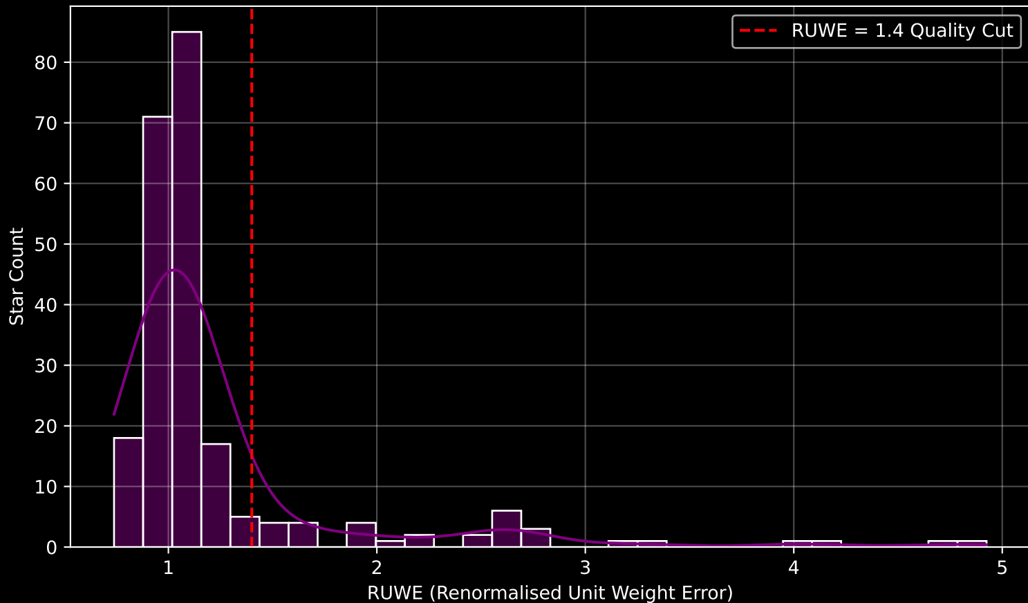
GALAH DR4 Field [7161] RUWE Distribution (n= 228)
